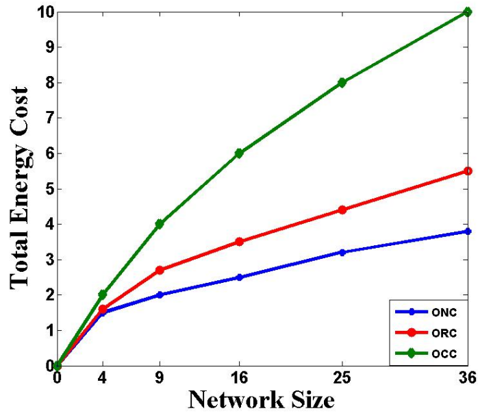
Figure 3.5: Total energy cost of optimal cooperative routing algorithms
