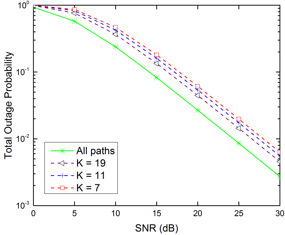
Figure 5.4: Total outage probability vs. SNR, for the Sub-optimal strategy with different numbers of paths, R_0 = 2 bps/Hz
