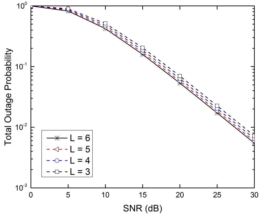
Figure 5.6: Total outage probability vs. SNR, for the L-relay ad-hoc strategy with different numbers of relays, R_0 = 2 bps/Hz
