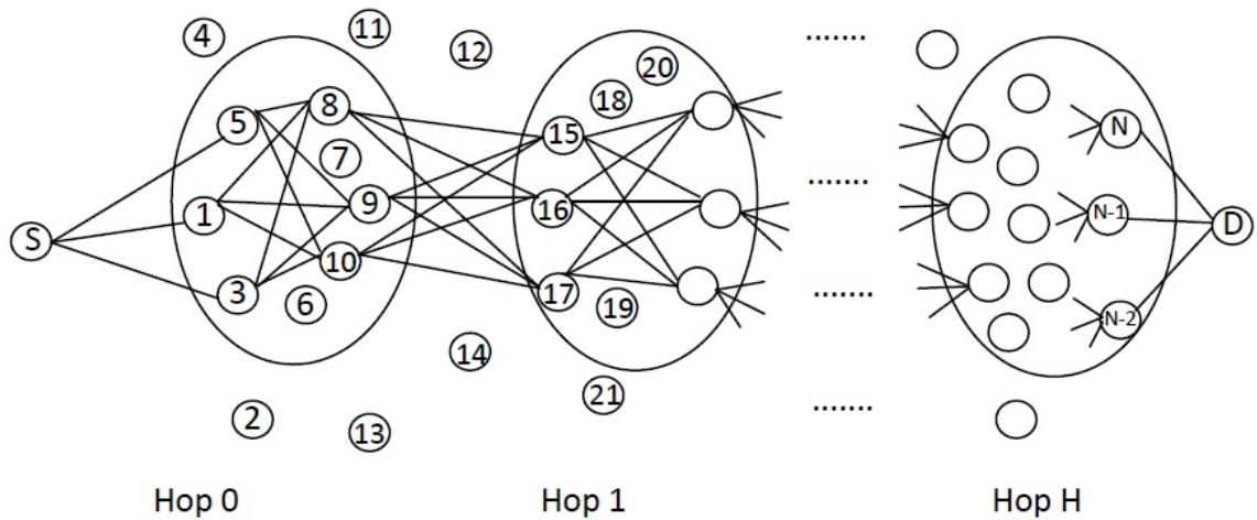
Figure 5.3: L-relay ad-hoc routing strategy cooperative network model
