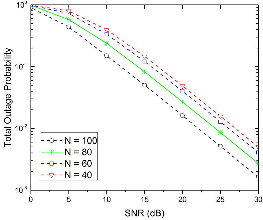
Figure 5.5: Total outage probability vs. SNR, for the Sub-optimal strategy with different number of nodes, R_0 = 2 bps/Hz
