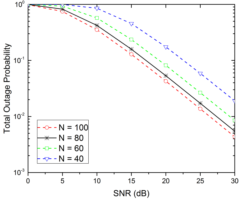
Figure 5.7: Total outage probability vs. SNR, for the Sub-optimal strategy with different number of nodes, R_0 = 2 bps/Hz
