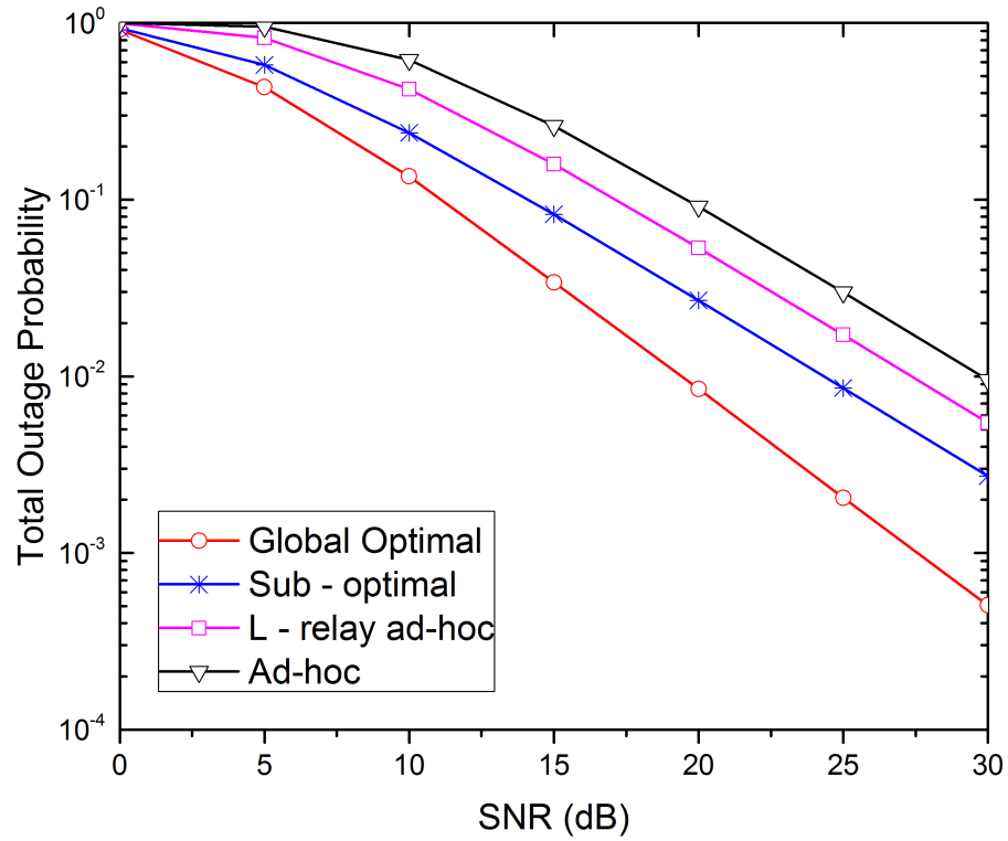
Figure 5.9: Total outage probability vs. SNR, for different routing strategies, R_0 = 2 bps/Hz
