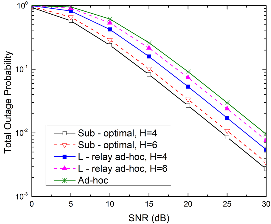
Figure 5.8: Total outage probability vs. SNR, with different number of hops, R_0 = 2 bps/Hz
