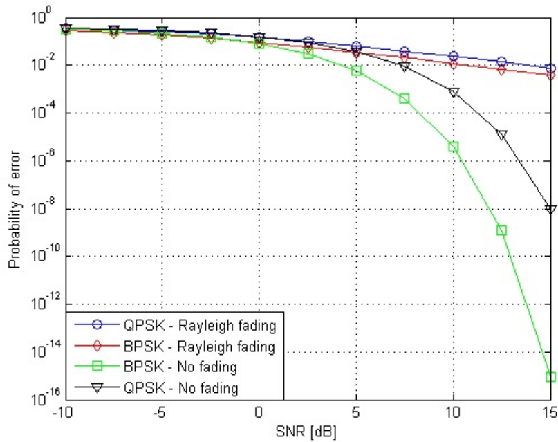
Figure A.1: Effects of Rayleigh Fading Channel
