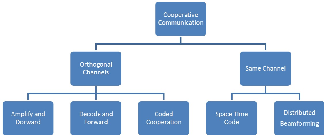
Figure 2.7: Various types of cooperative communications
