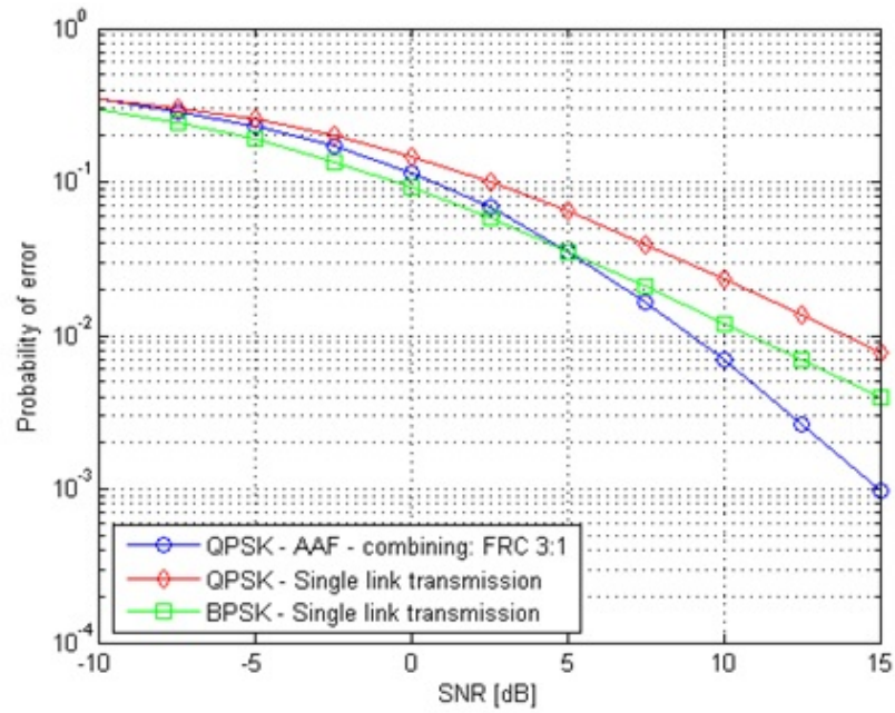
Figure A.5: Amplify and Forward method using BPSK vs Direct transmission
