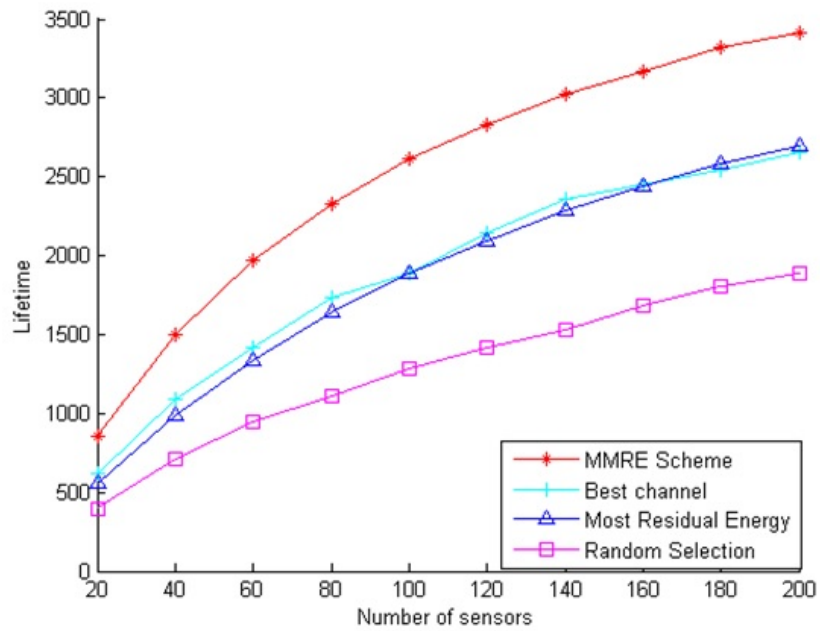
Figure A.6: Lifetime under different non-cooperative protocols
