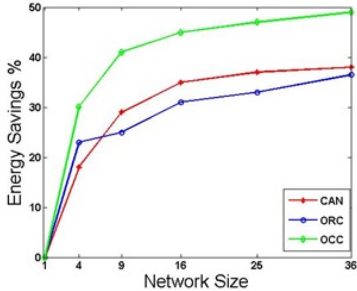
Figure 3.6: Energy savings of optimal cooperative routing algorithms
