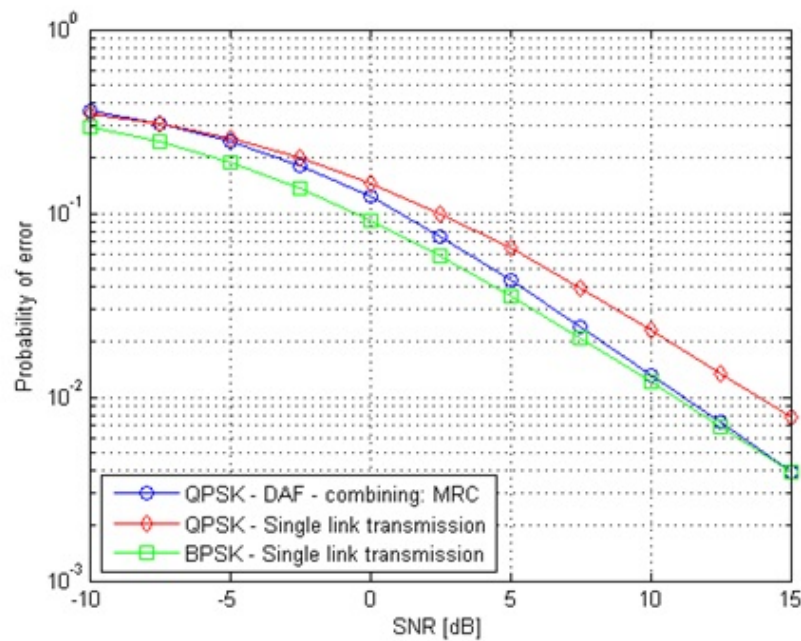
Figure A.2: Decode and Forward method using QPSK vs Direct transmission
