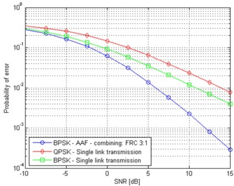
Figure A.4: Amplify and Forward method using BPSK vs Direct transmission
