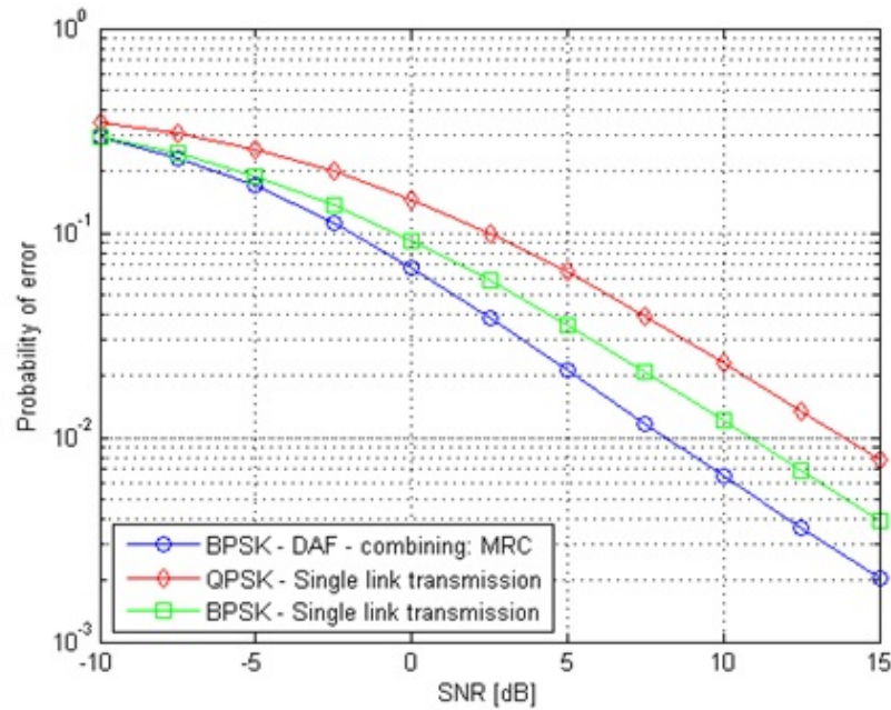
Figure A.3: Decode and Forward method using BPSK vs Direct transmission
